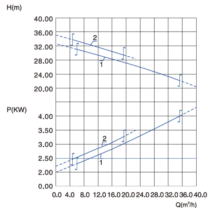
泵性能曲线图 Pump performance curve chart
