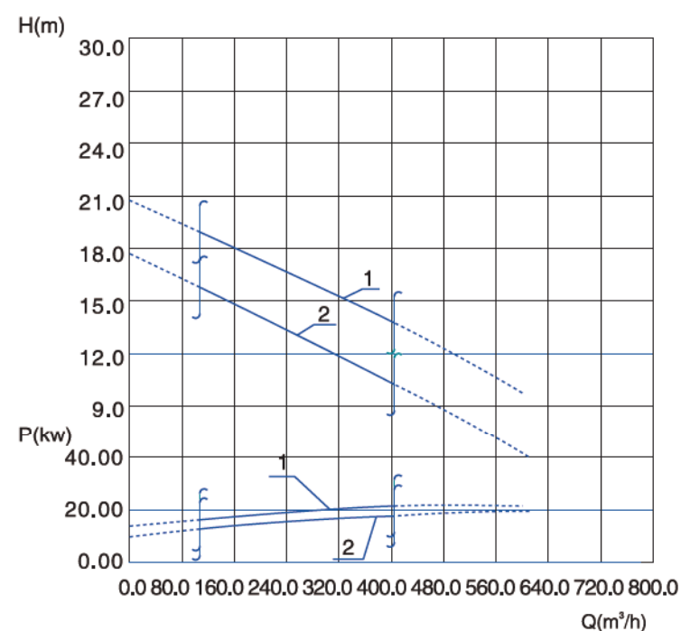
Example 2 of performance curve chart and main parameters
