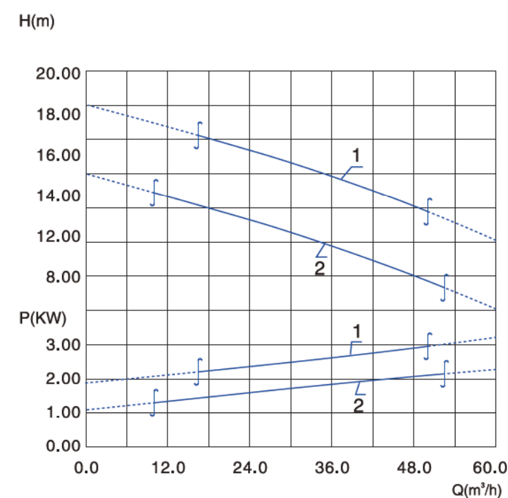
泵性能曲线图 Pump performance curve chart
