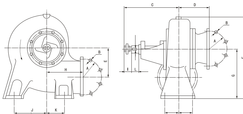
图5 400HW~800HW和350HW-8泵水平出水外形安装图 (650HW型泵的出水方向和叶轮转向与图示相反) Fig.5 Out-form and installation diagram of model 150~300HW and 350HW-8 pump with the water out horizontally (both water out direction and impeller moving direction of model 650HW pump are reversed to that shown in the figure)
